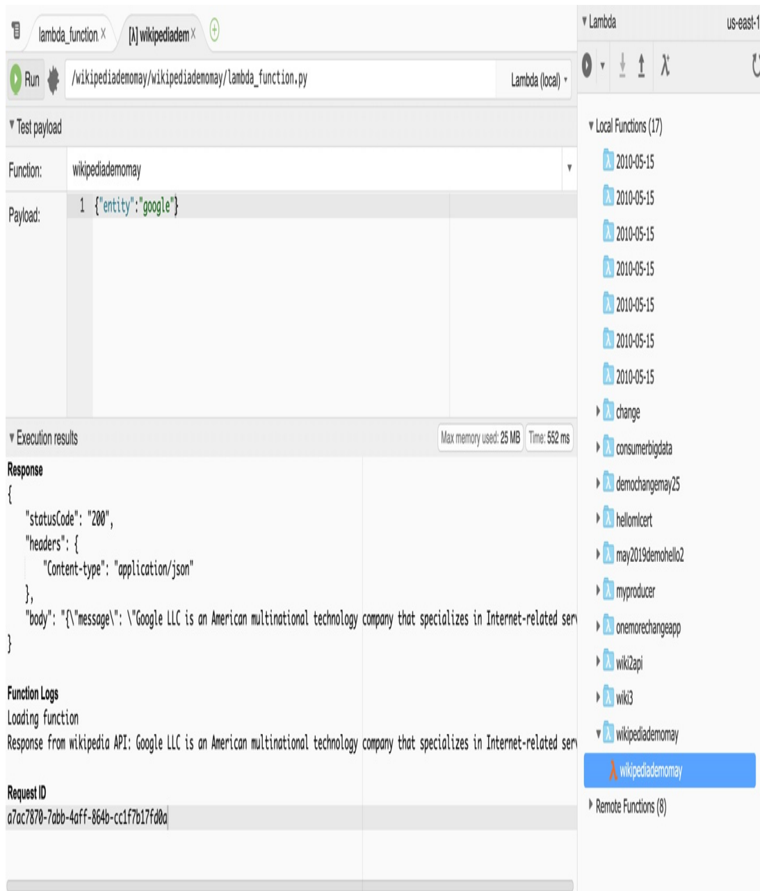
Figure 9-4. Running Lambda Function in Cloud9
