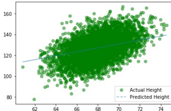
Figure 14-5. Predicted height versus actual height
