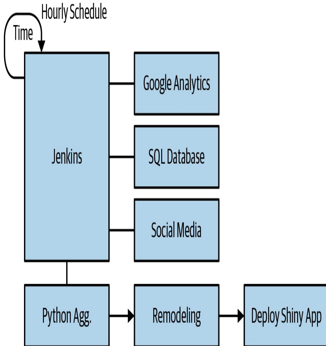
Figure 15-6. Jenkins data pipeline
