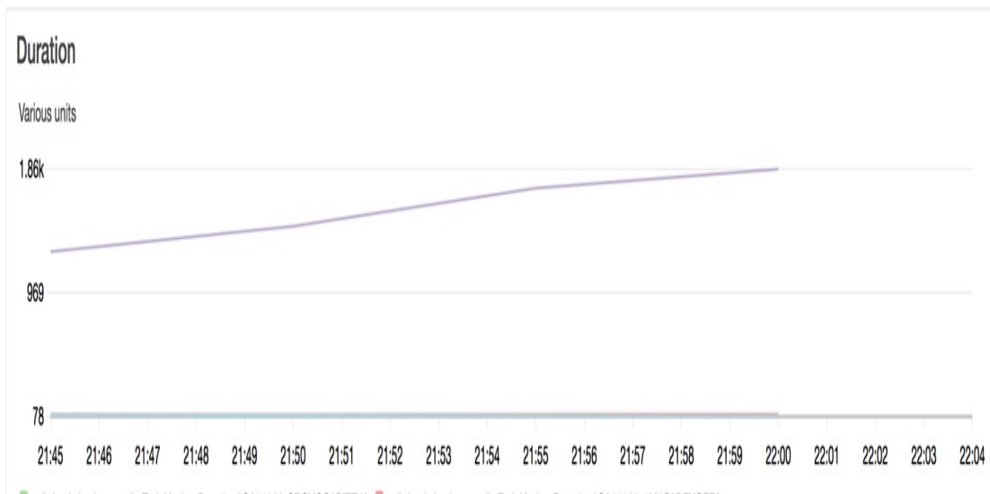
Figure 13-6. Lambda duration
