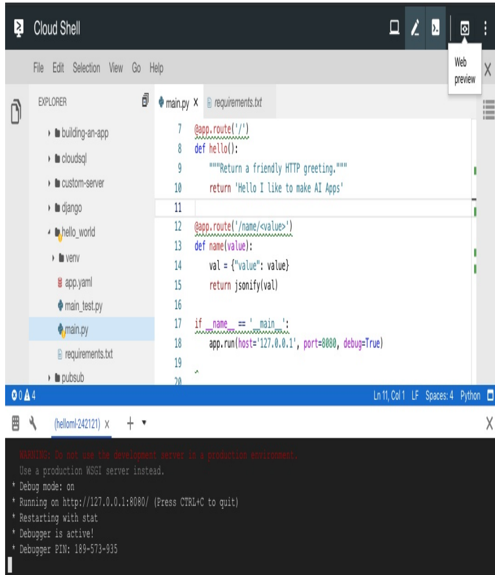
Figure 6-2. Web preview
