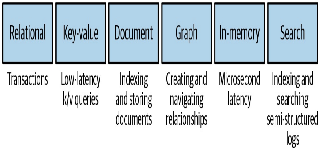
Figure 15-4. Amazon databases
