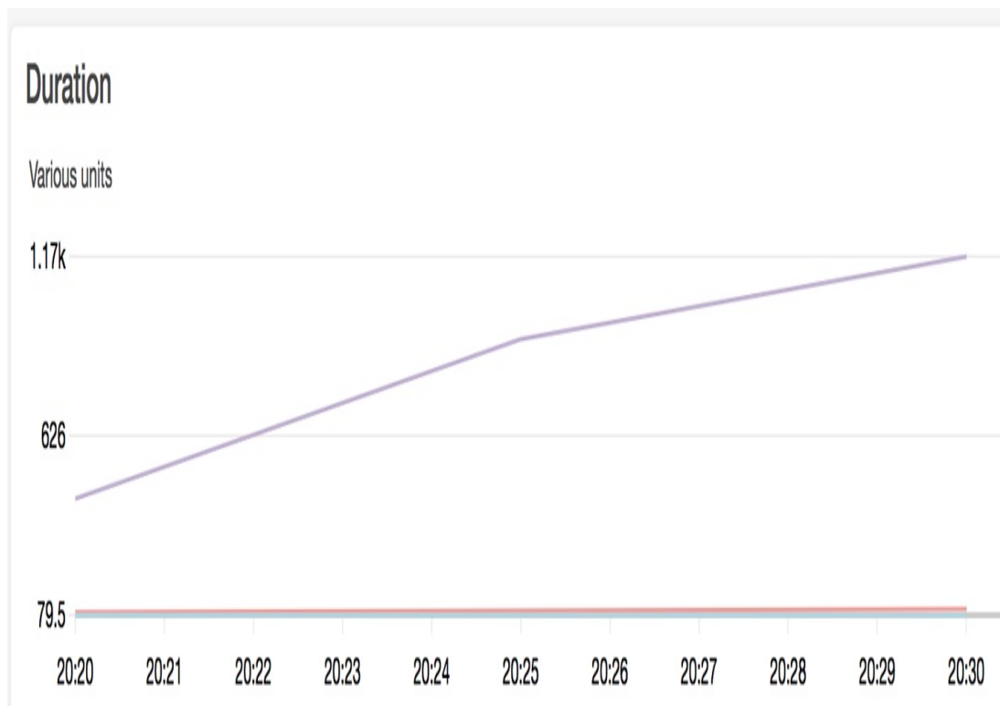
Figure 13-3. Lambda duration
