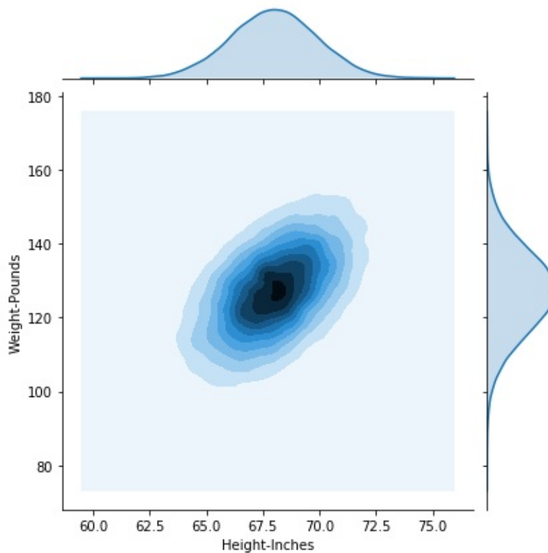
Figure 14-2. Density plot
