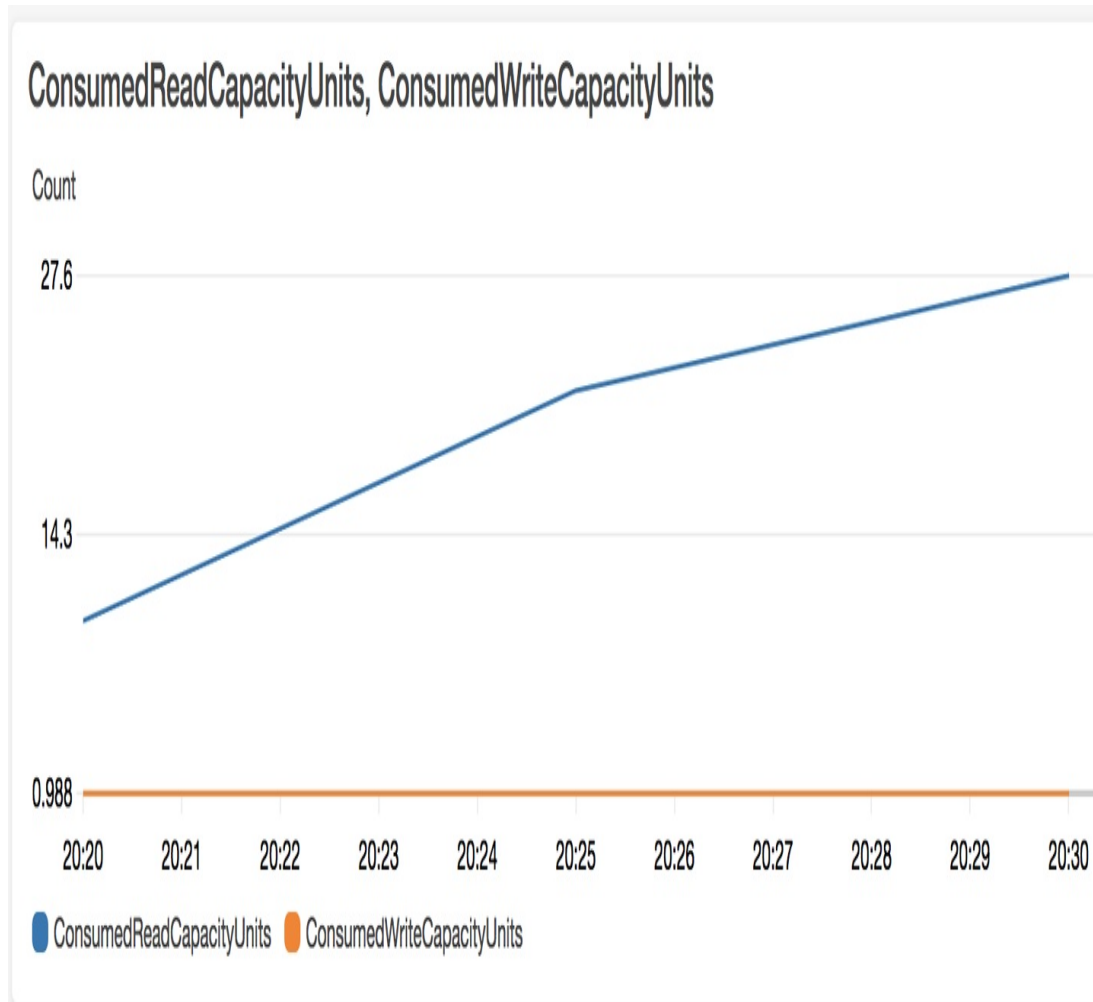
Figure 13-4. DynamoDB consumed read and write capacity units
