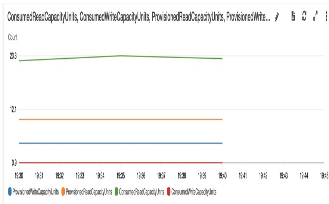
Figure 13-2. DynamoDB provisioned and consumed read and write capacity units
