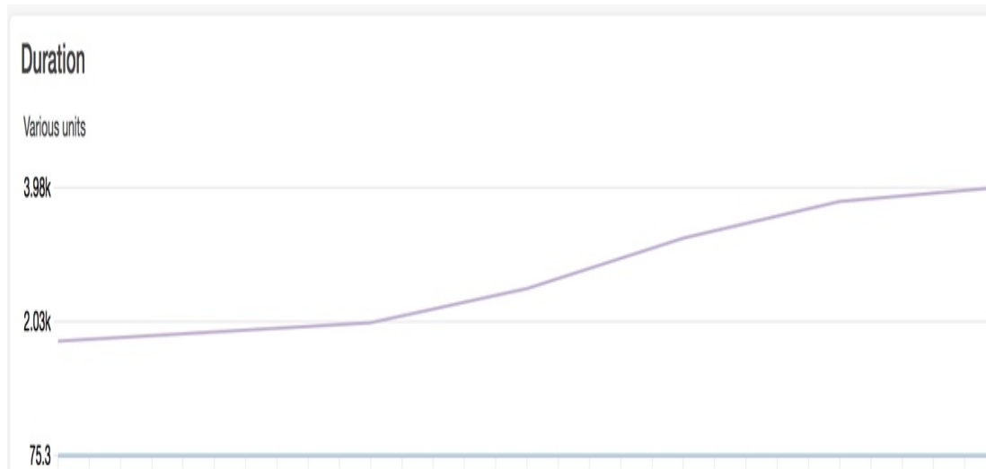
Figure 13-8. Lambda duration
