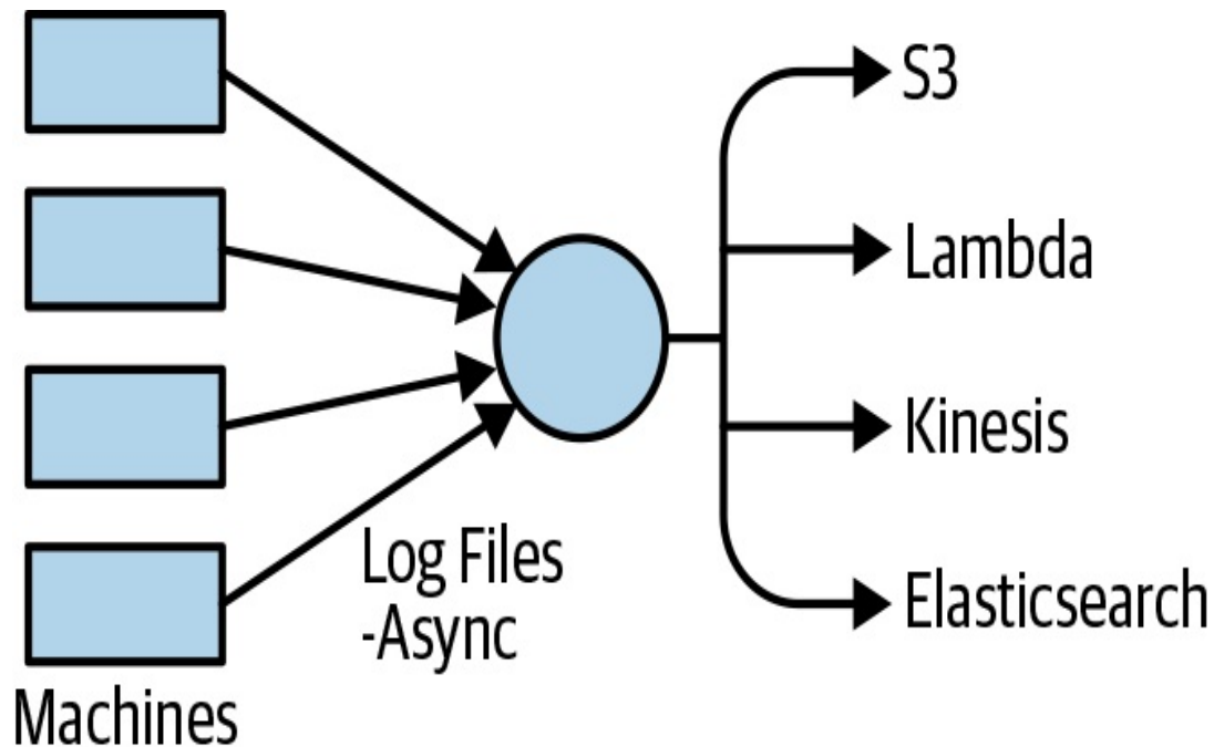
Figure 15-5. Kinesis log files
