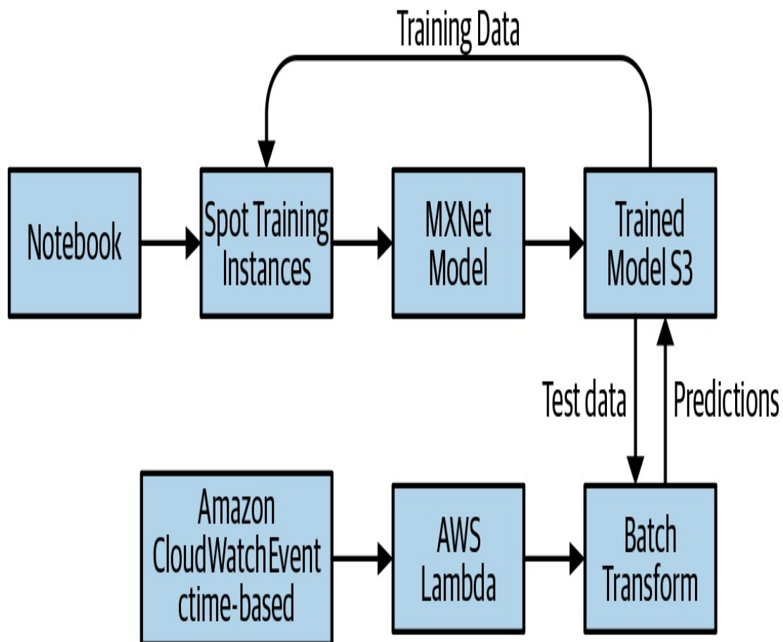
Figure 14-7. Amazon SageMaker
