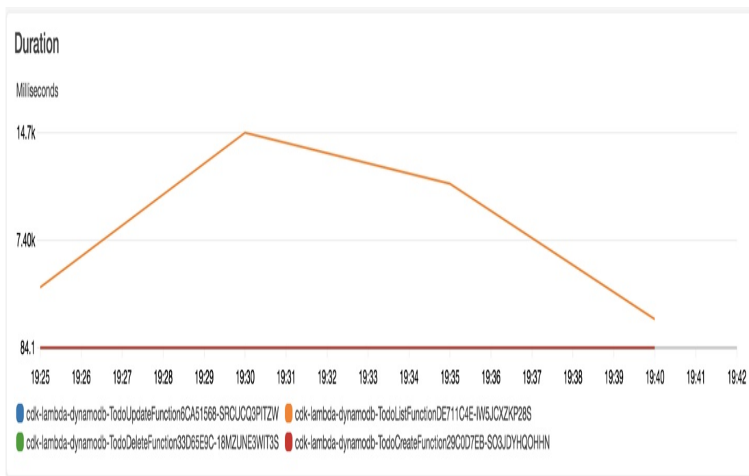
Figure 13-1. Lambda duration
