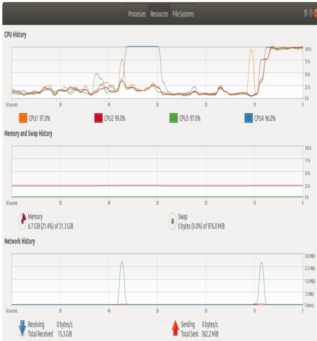
Figure 3-1. Using all of the cores
