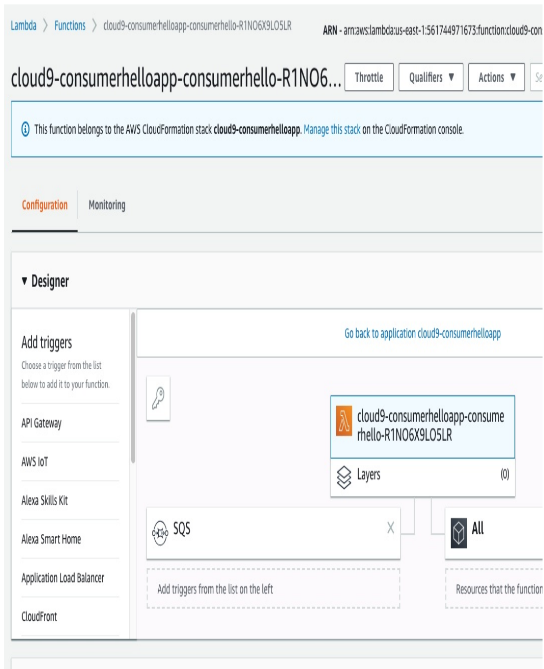
Figure 15-15. Fire on SQS event
