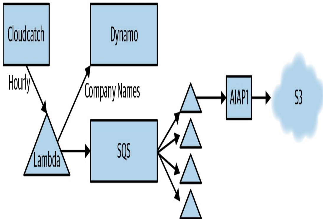
Figure 15-7. Serverless data pipeline
