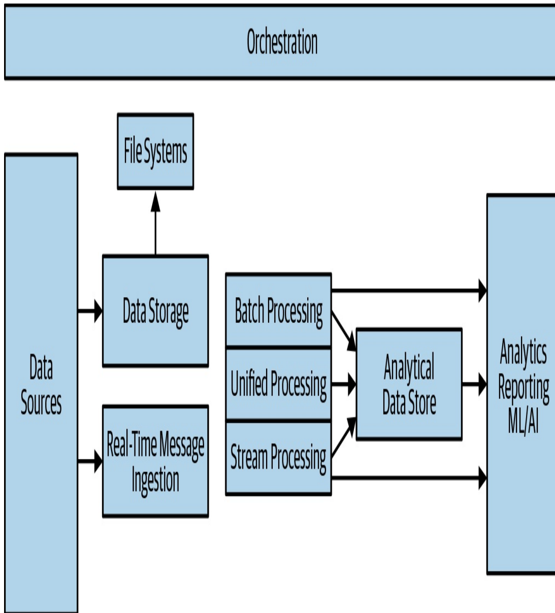
Figure 15-1. Big Data architecture
