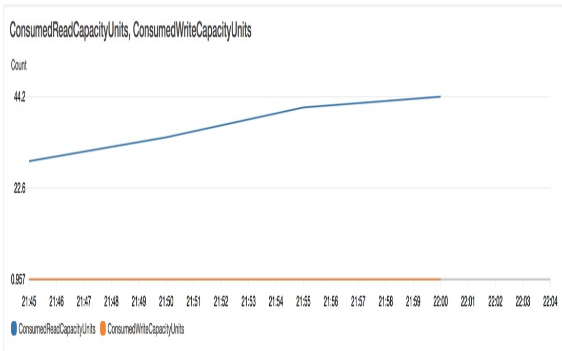
Figure 13-7. DynamoDB consumed read and write capacity units
