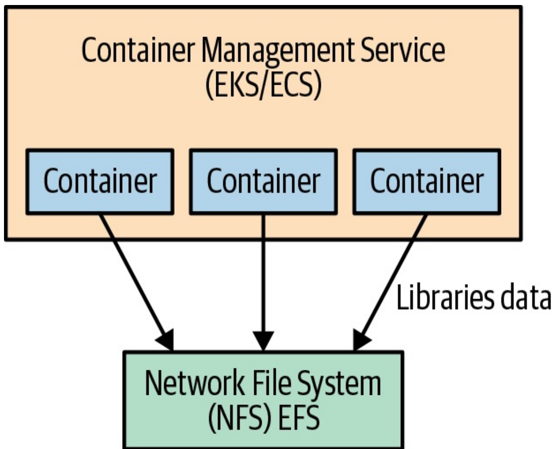
Figure 15-2. Mounting EFS in a container
